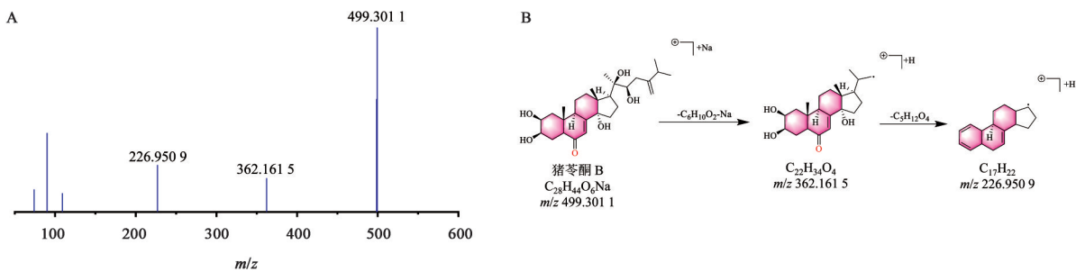
图6 猪苓酮B的质谱裂解途径 Fig. 6 MS cracking pathways of polyporusterone B
